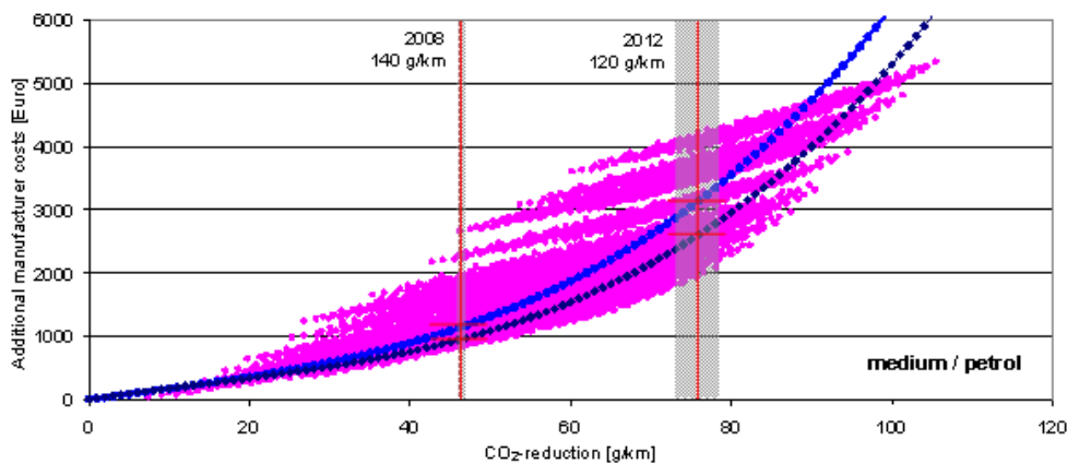
Figure 4 - Assessment of the impact of a different “safety margin” in drawing the cost curves on the costs of CO 2 -reductions required to meet the 2008/9 and 2012 targets (example for medium petrol vehicle)
